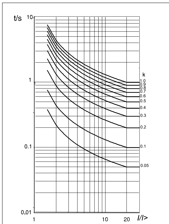
Normal Inverse 1.3/10
