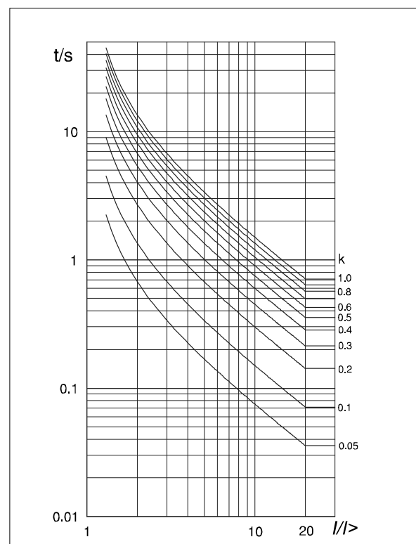
Very Inverse
