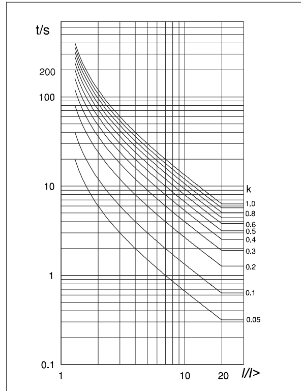
Long-time Inverse
